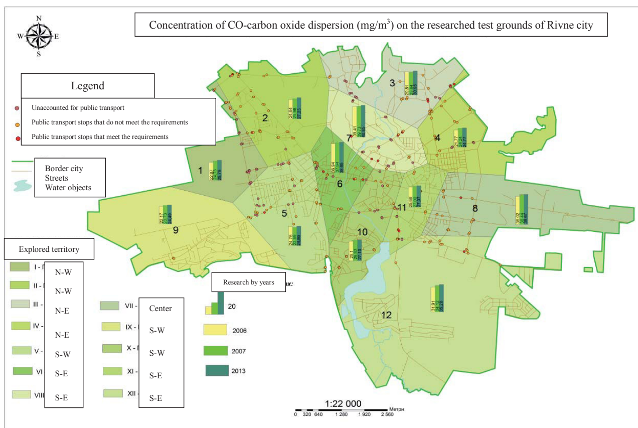
Figure 2. Concentration of CO-carbon oxide dispersion ( \text{mg}/\text{m}^3 ) on the researched test grounds of Rivne city
