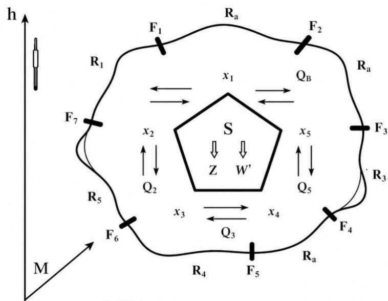
Figure 1. Formalized model of a natural-technogenic aquatic ecosystem
